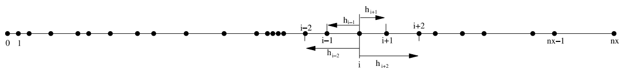
Fig. 4. Nonuniform grid with nx + 1 grid points distributed arbitrarily.
