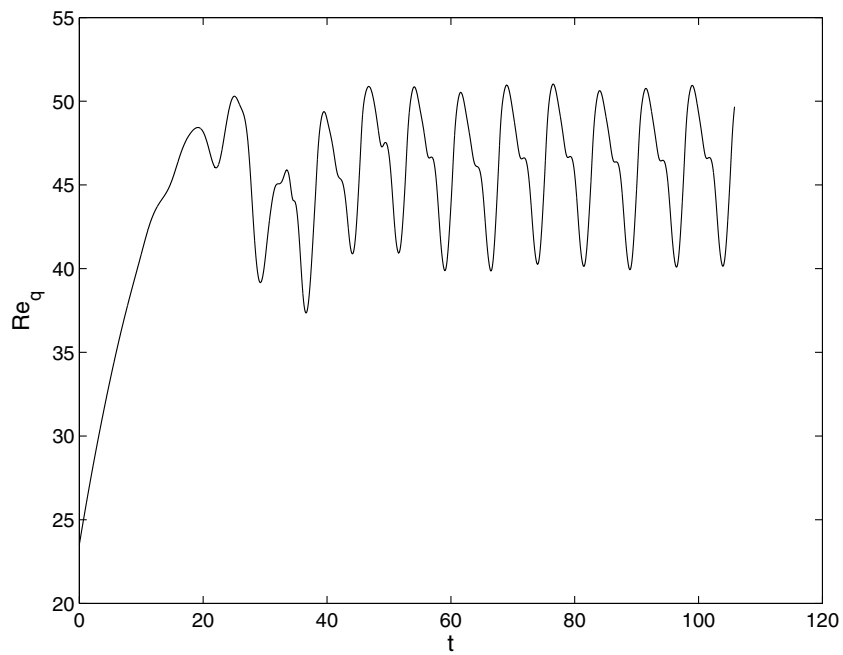
Fig. 11. Reynolds number based on the exit flow rate as a function of time.
