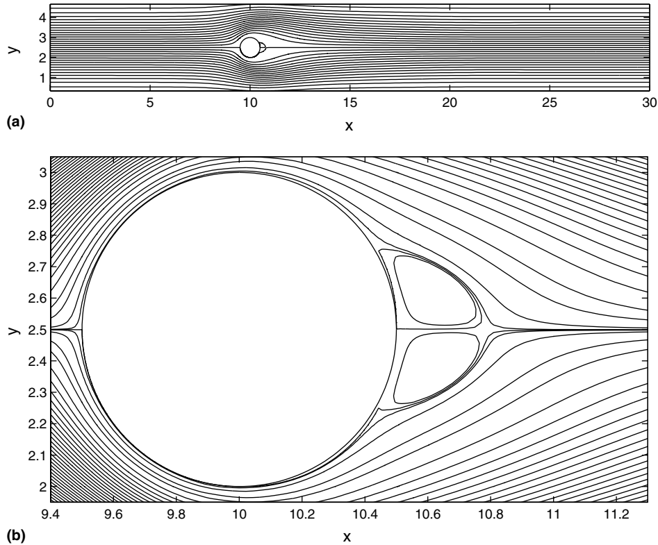
Fig. 13. Flow inside a channel with a single circular cylinder for Re_q = 10 . (a) Streamlines (all the lengths are scaled with the diameter of the cylinder). (b) Detail of the wake behind the cylinder.
