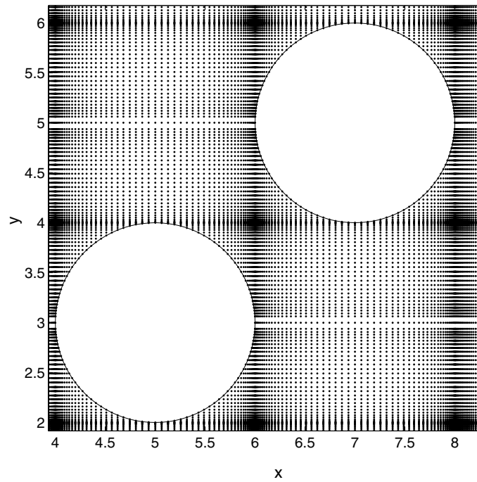
Fig. 10. Mesh points concentrated around the cylinders.
